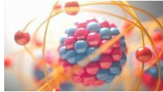
Atoms & Molecules
